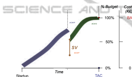
Figure 3: EVM metrics.
