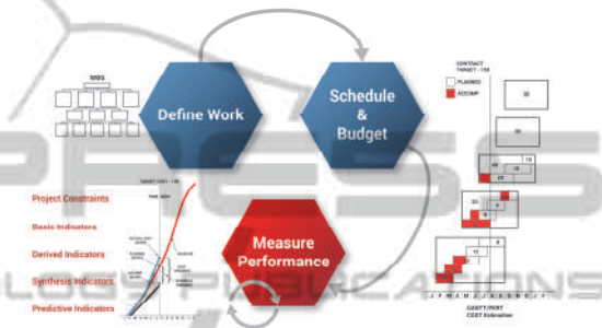
Figure 2: Project phases.
